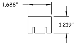
BOTTOM RAIL
