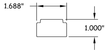
1" STILE/TOP RAIL
